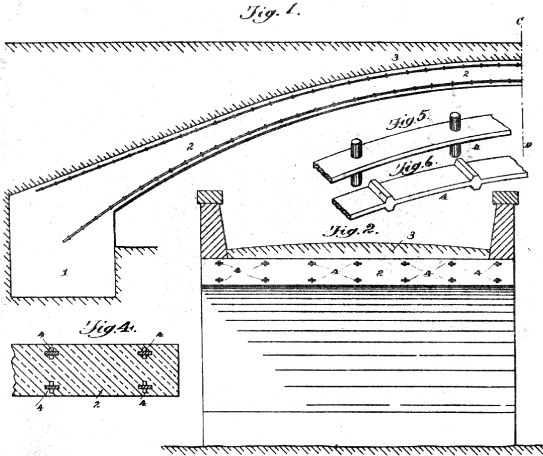
Figure 11. Edwin Thacher's Reinforcing System (which used two tiers of deformed steel bars; this design was widely used after the patent was voided in 1916)
