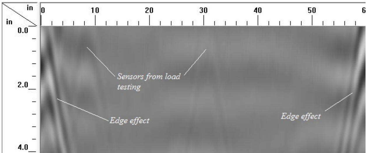
Figure 25. Ground Penetrating Radar Scan of Bottom Flange With No Moisture
