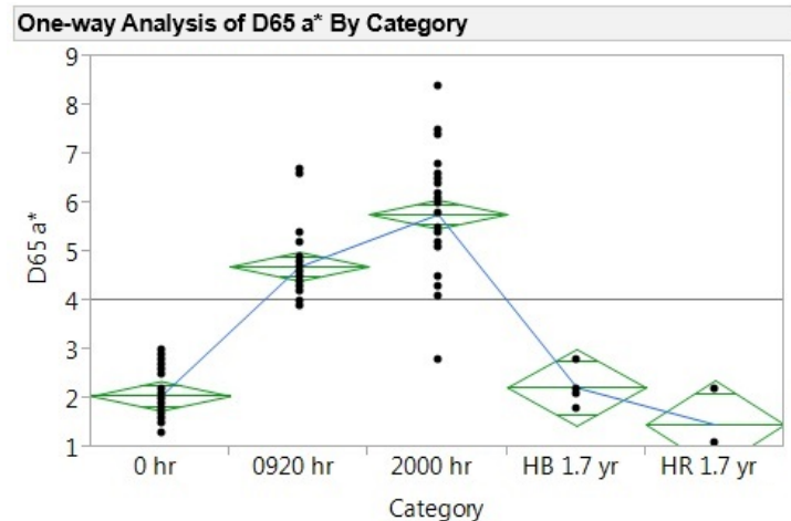
Figure 21. Statistical Means Comparison for D65 a* Values of Laboratory and Field Specimens
